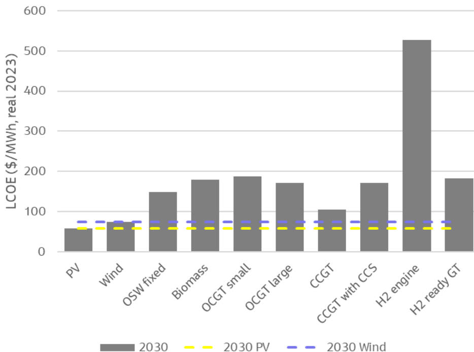
Figure 3-4. LCOE of various generating technologies in Victoria
